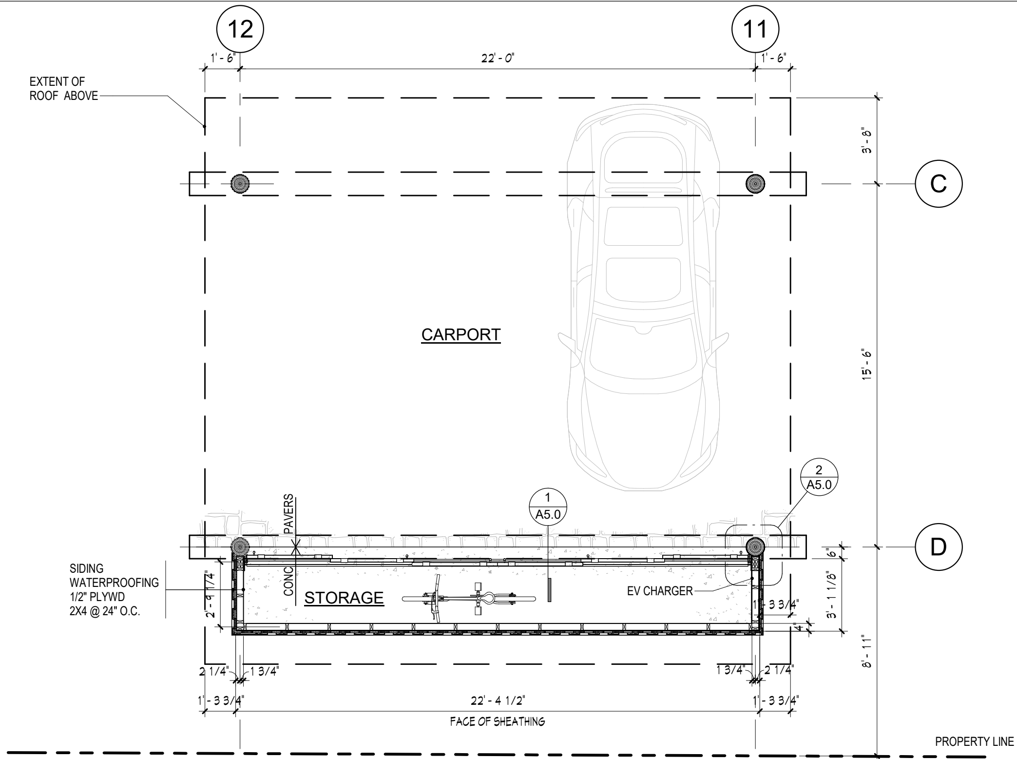
Floor Plan 1 SCALE: 1/4" = 1'-0"
