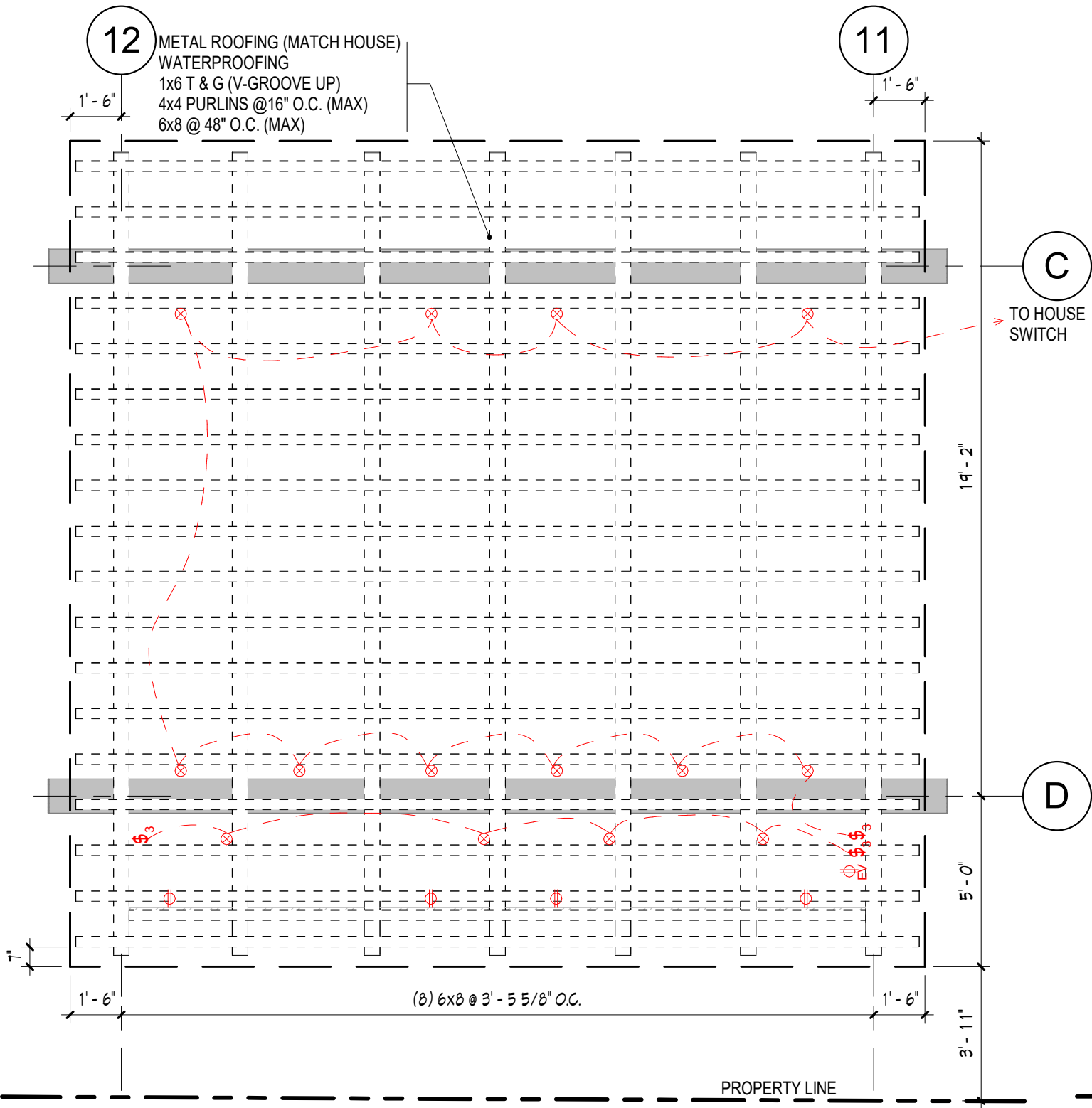
Roof Framing & Electrical Plan SCALE: 1/4" = 1'-0" 2
