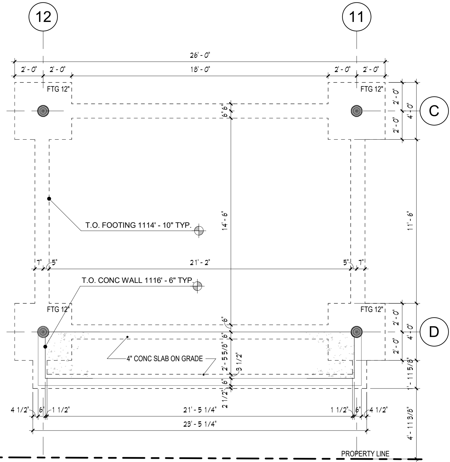
Foundation Plan SCALE: 1/4" = 1'-0" 1
